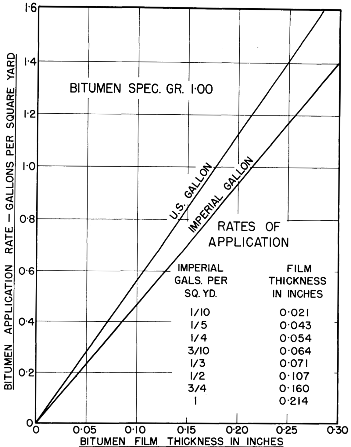
FIG. 10 RELATIONSHIP BETWEEN BITUMEN FILM THICKNESS AND GALLONS PER SQUARE YARD.
