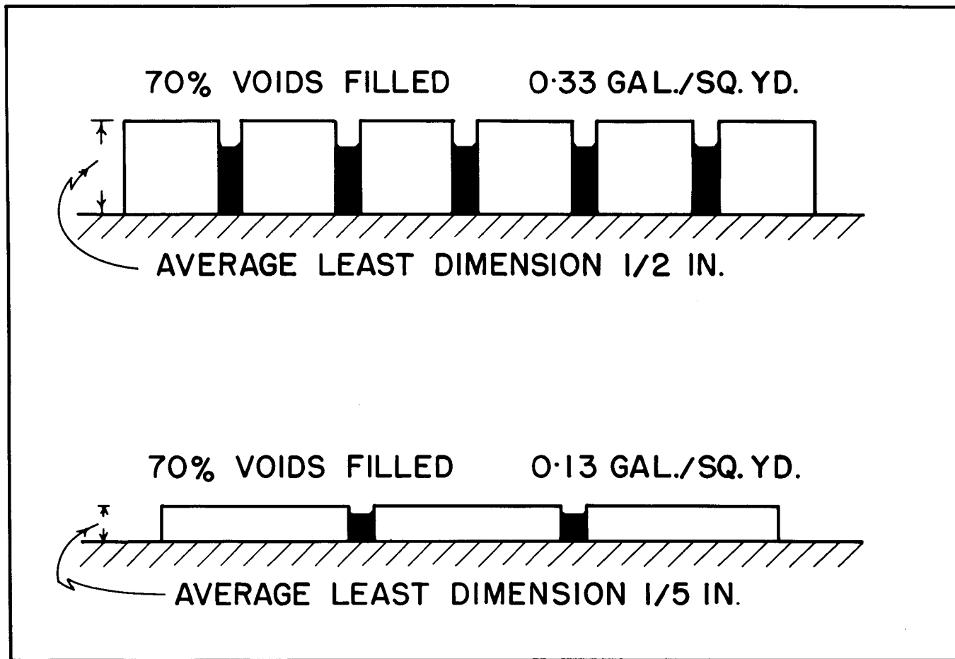
FIG.12 COMPARING BITUMEN REQUIREMENTS FOR SEAL COATS MADE WITH 1/2 INCH COVER AGGREGATES OF DIFFERENT PARTICLE SHAPES — ONE CUBICAL, THE OTHER FLAT AND ELONGATED.
