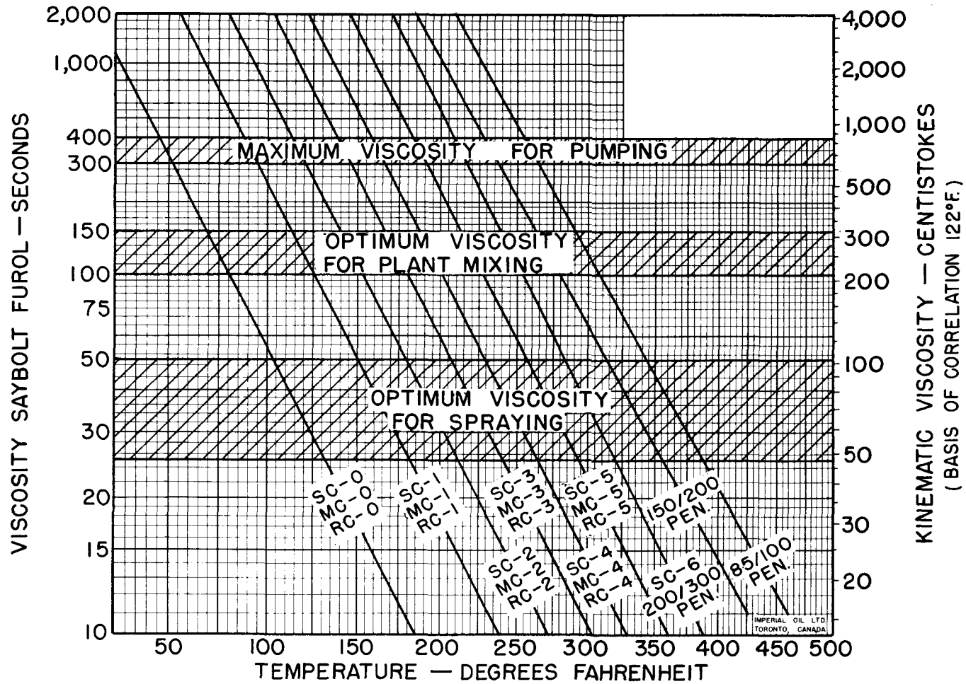
FIG.3 ILLUSTRATING RECOMMENDED VISCOSITIES FOR SPRAYING AND MIXING ASPHALT PRODUCTS, AND MAXIMUM VISCOSITIES FOR PUMPING.
