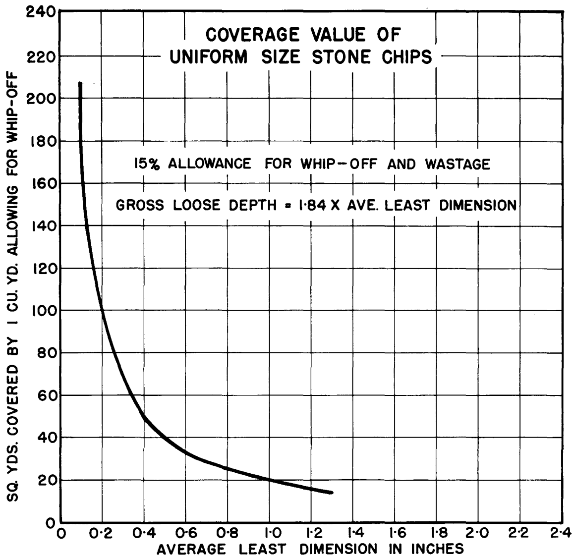
FIG. 9 RELATIONSHIP BETWEEN AVERAGE LEAST DIMENSION AND COVERAGE VALUE WITH ALLOWANCE FOR WHIP-OFF AND WASTAGE.
