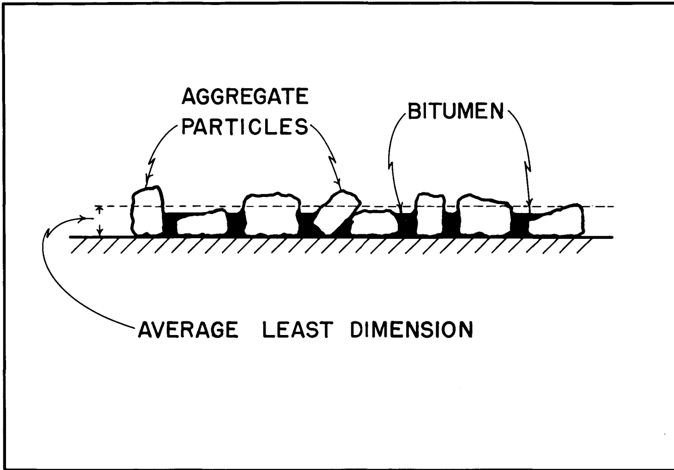
FIG. 6 ILLUSTRATING THE AVERAGE LEAST DIMENSION OF THE COVER AGGREGATE FOR A SEAL COAT OR SURFACE TREATMENT.
