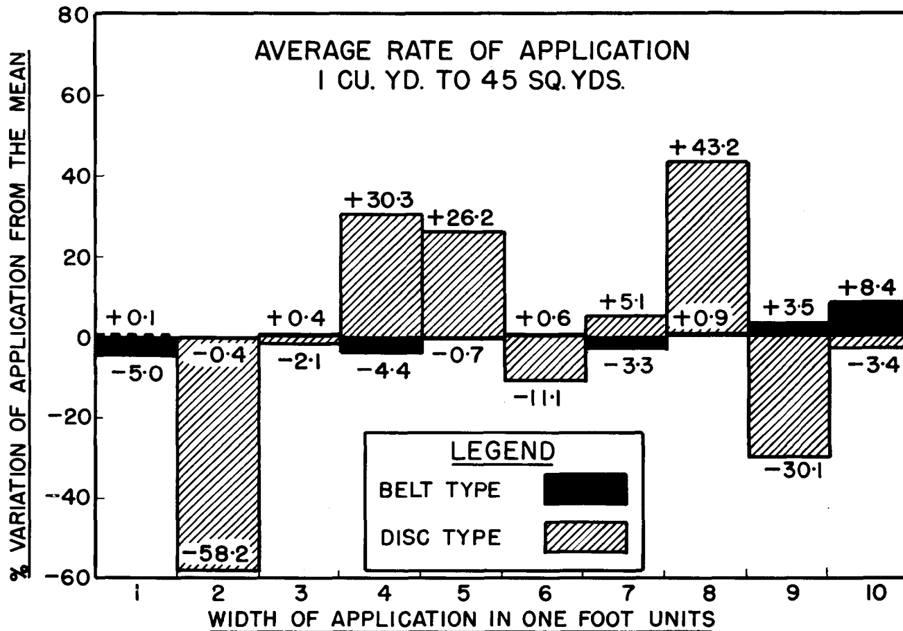
FIG. 5 COMPARISONS OF VARIATIONS IN TRANSVERSE DISTRIBUTION OBTAINED WITH A ROTATING DISC SPREADER AND A BELT SPREADER (AGGREGATE MAXIMUM SIZE 5/8 IN. — AVERAGE RATE OF APPLICATION 1 CU. YD. TO 45 SQ. YDS.)
