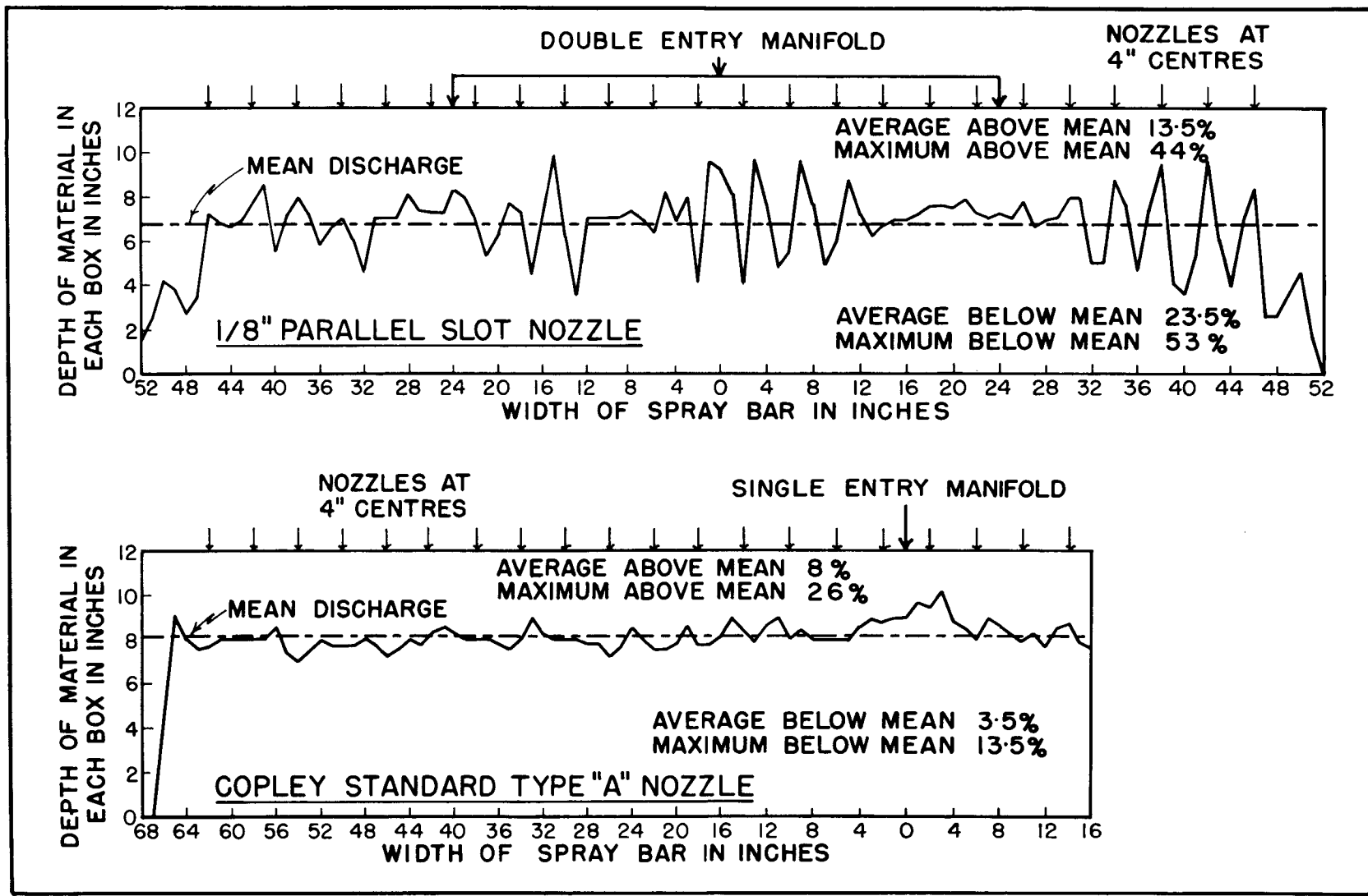
FIG. 4 COMPARISON OF DISCHARGE FROM TWO TYPES OF SPRAY NOZZLES
