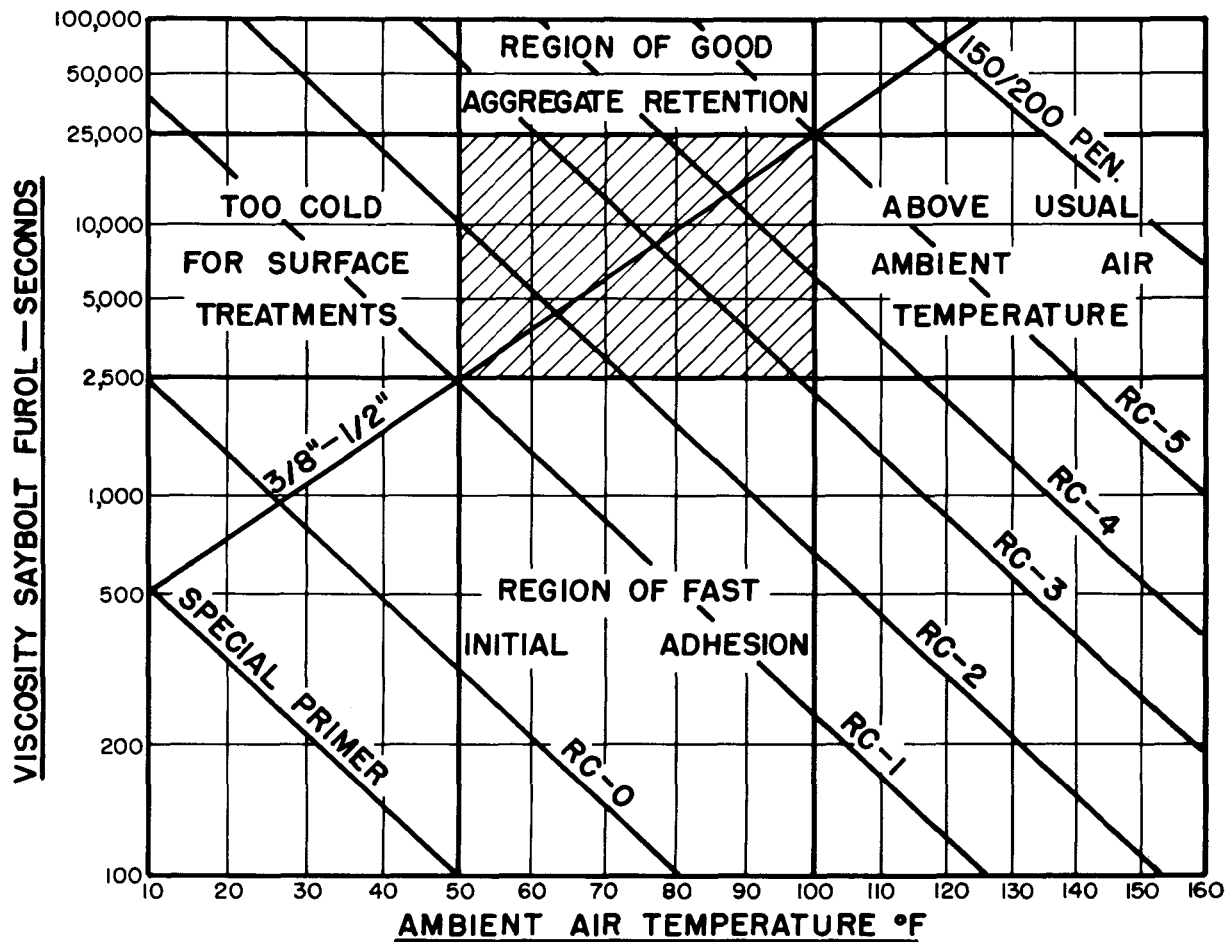
FIG.13 INFLUENCE OF INITIAL ADHESION, RESISTANCE TO DISPLACEMENT BY TRAFFIC, AND AMBIENT AIR TEMPERATURES ON SELECTION OF ASPHALT BINDER (3/8" TO 1/2" COVER AGGREGATE)
