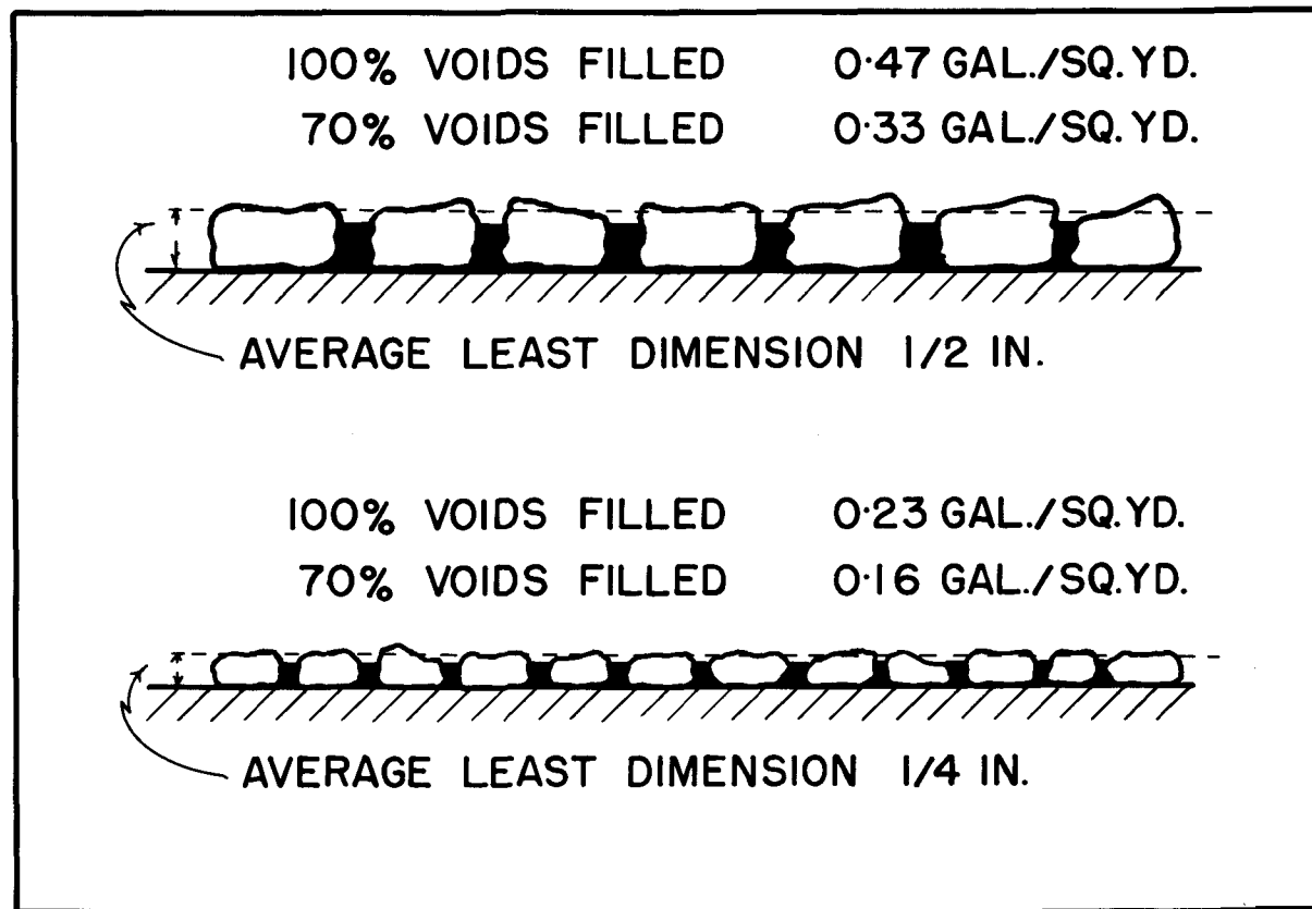
FIG. II ILLUSTRATING THAT SURFACE TREATMENTS MADE WITH LARGER AGGREGATES ARE LESS SENSITIVE TO SMALL VARIATIONS IN BITUMEN APPLICATION THAN WHEN SMALLER COVER AGGREGATES ARE USED.
