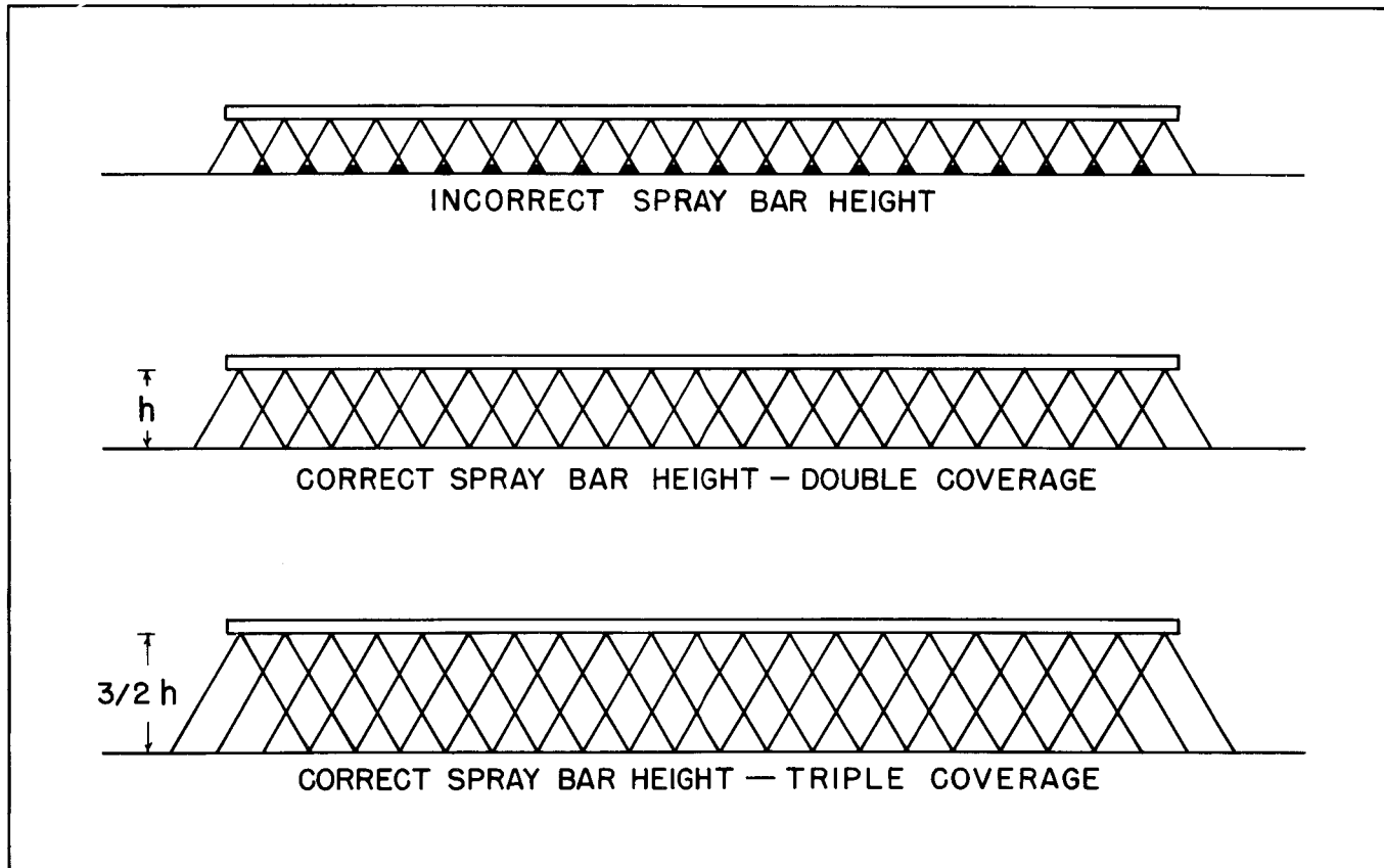
FIG.2 INFLUENCE OF SPRAY BAR HEIGHT
