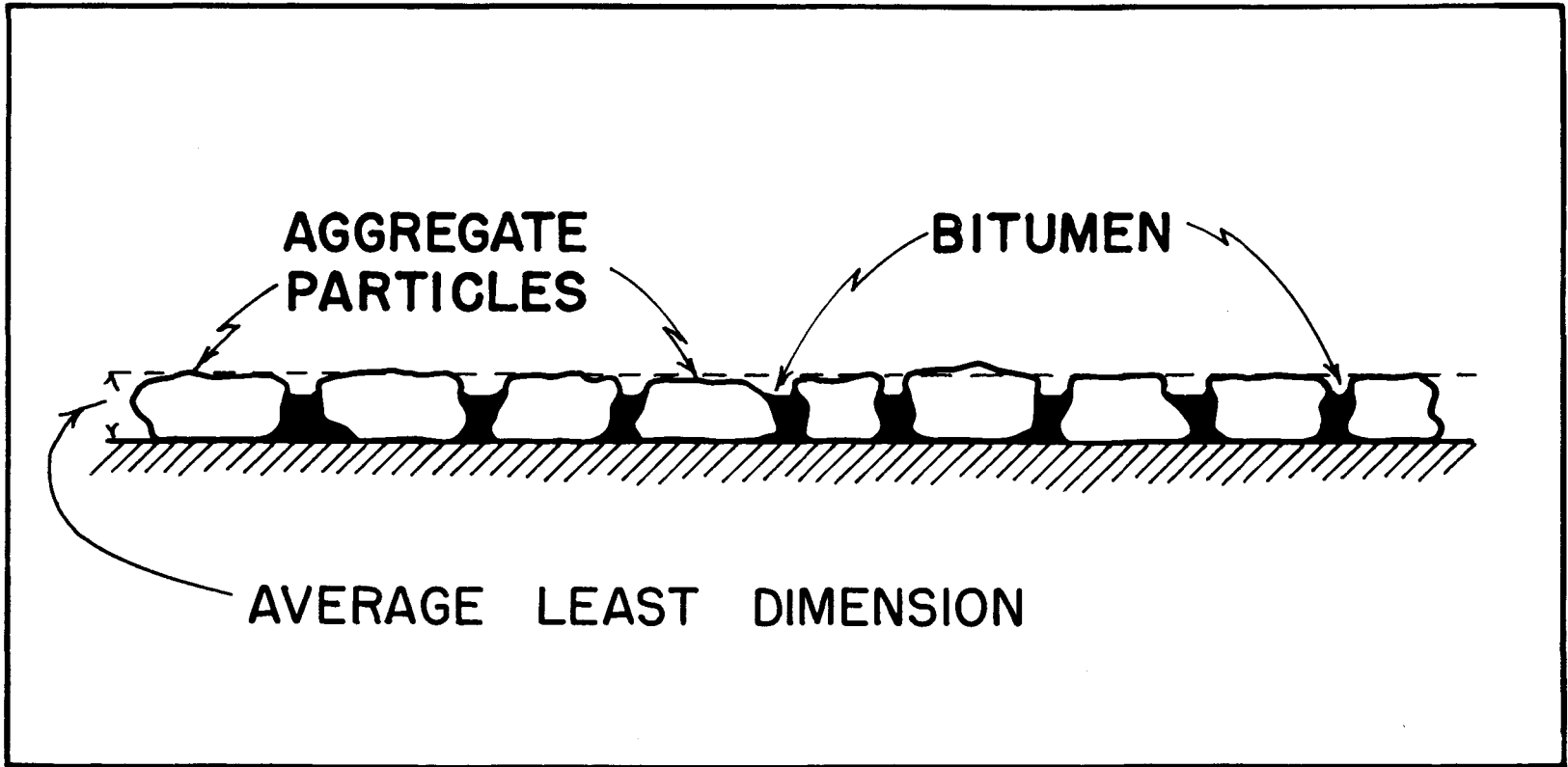
FIG. 7 PROPERLY CONSTRUCTED SURFACE TREATMENT OR SEAL COAT.
